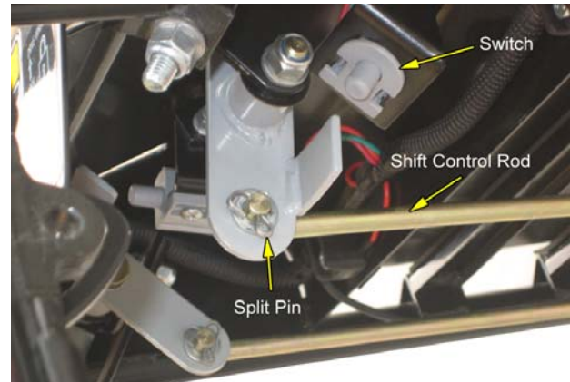
FIG 13 Shift Control Rod Adjustment
