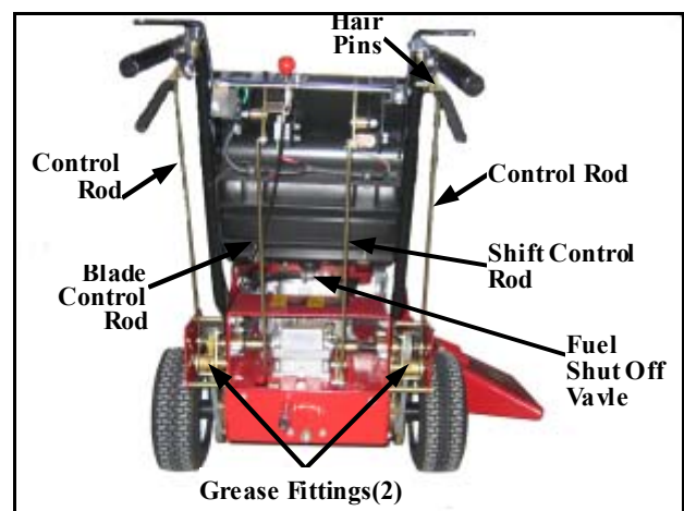
FIG 10 Wheel Drive Controls
