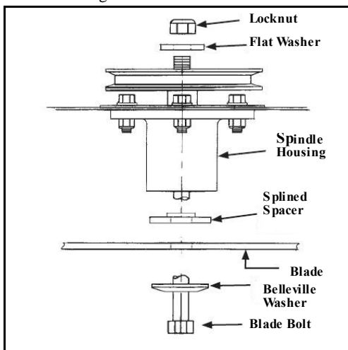
FIG 5 Mower Spindle & Blades
