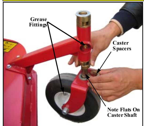
FIG 14 Repositioning Caster Spacers
