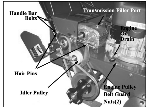
FIG 9 Wheel Drive Belts
