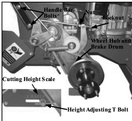
FIG 11 Brake Linkage
