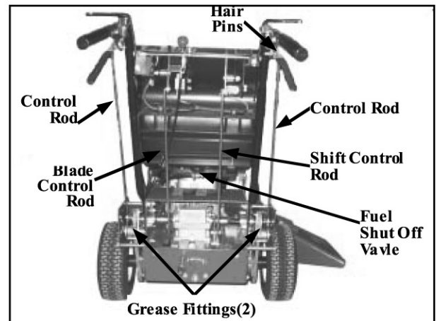
FIG 10 Wheel Drive Controls
