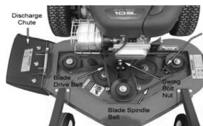
FIG 7 Blade Drive Belt
