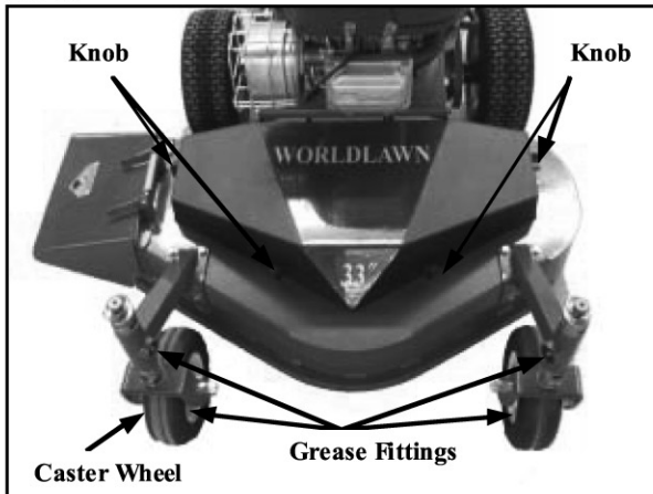
FIG 4 Belt Cover
